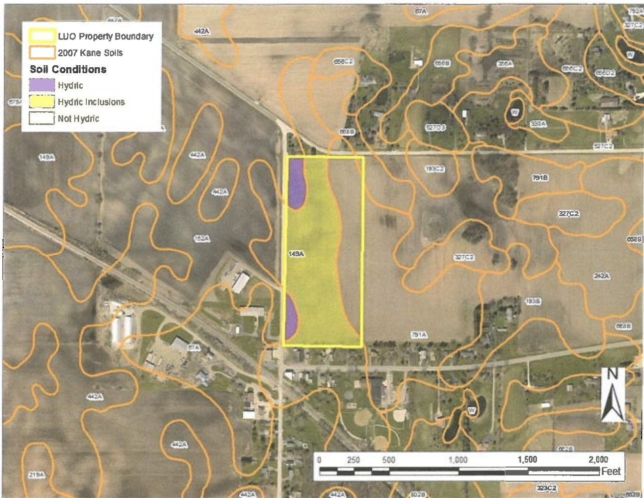
Figure 9: Hydric Soils
