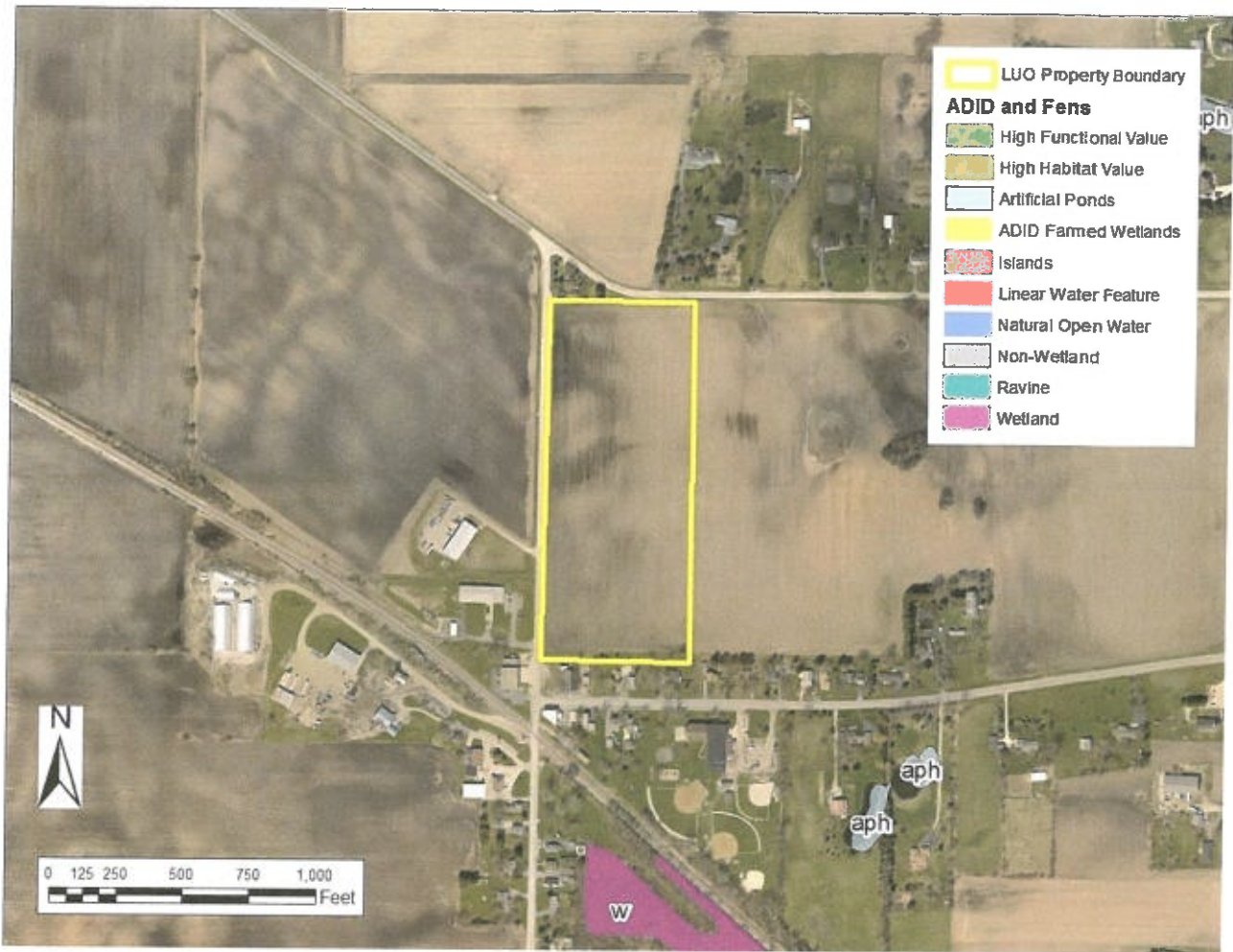
Figure 4: ADID Wetlands
